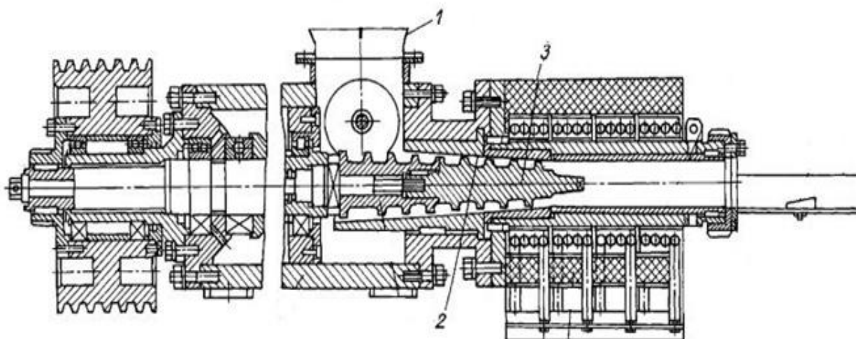
Figure 3. Auger press: 1 - place of raw material loading; 2 - drum; 3 – auger
