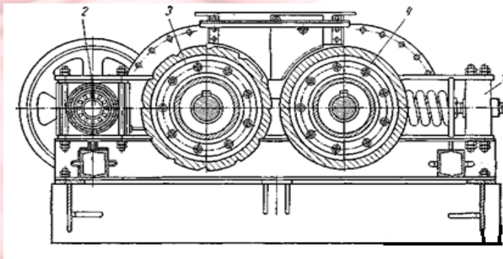
Figure 1. Two-wheel gear grinder: 1 - spring; 2 - gear extension; 3, 4 - gears.
