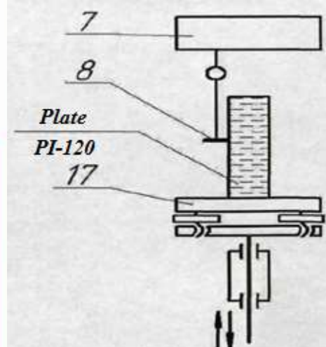
Fig. 2. Scheme of checking the error of axial displacement.
