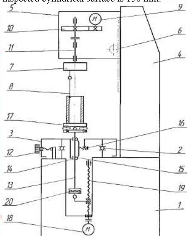
Fig. 1. Kinematic diagram of modernized BE-20A roundness gauge.
